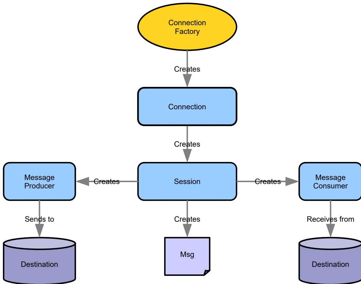
Illustration 1: Programming Model
